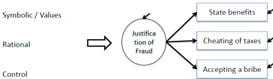
Figure 2: Theoretical model
